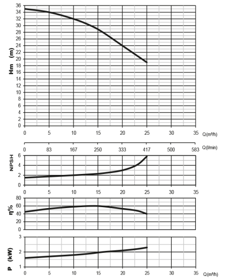
SMINOX160/32 2.2 KW
