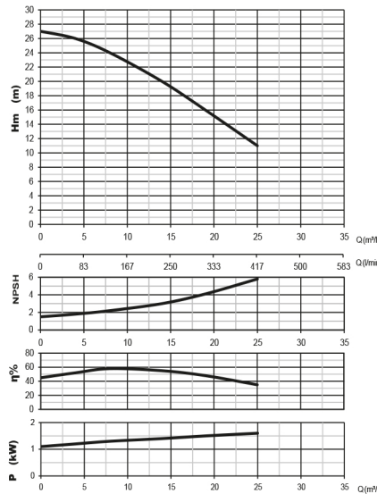
SMINOX160/32 1.5 KW
